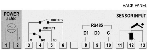
Figure 1 – N322 terminals
